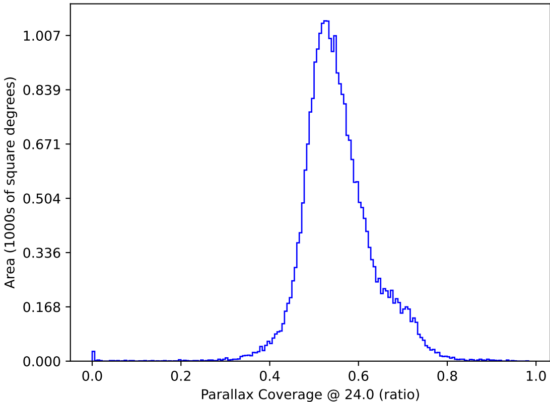
too_elab_r64_d3_gz_v3.4_10yrs : Parallax Coverage @ 24.0
