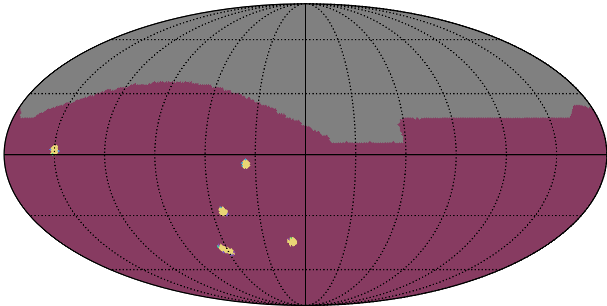
too_elab_r64_d3_gz_v3.4_10yrs : NumberOfQuickRevisits
