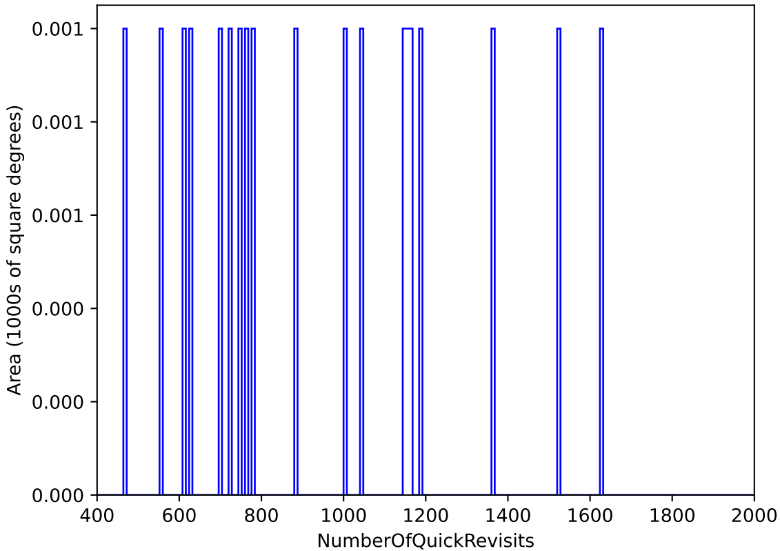
too_elab_r64_d3_gz_v3.4_10yrs : NumberOfQuickRevisits
