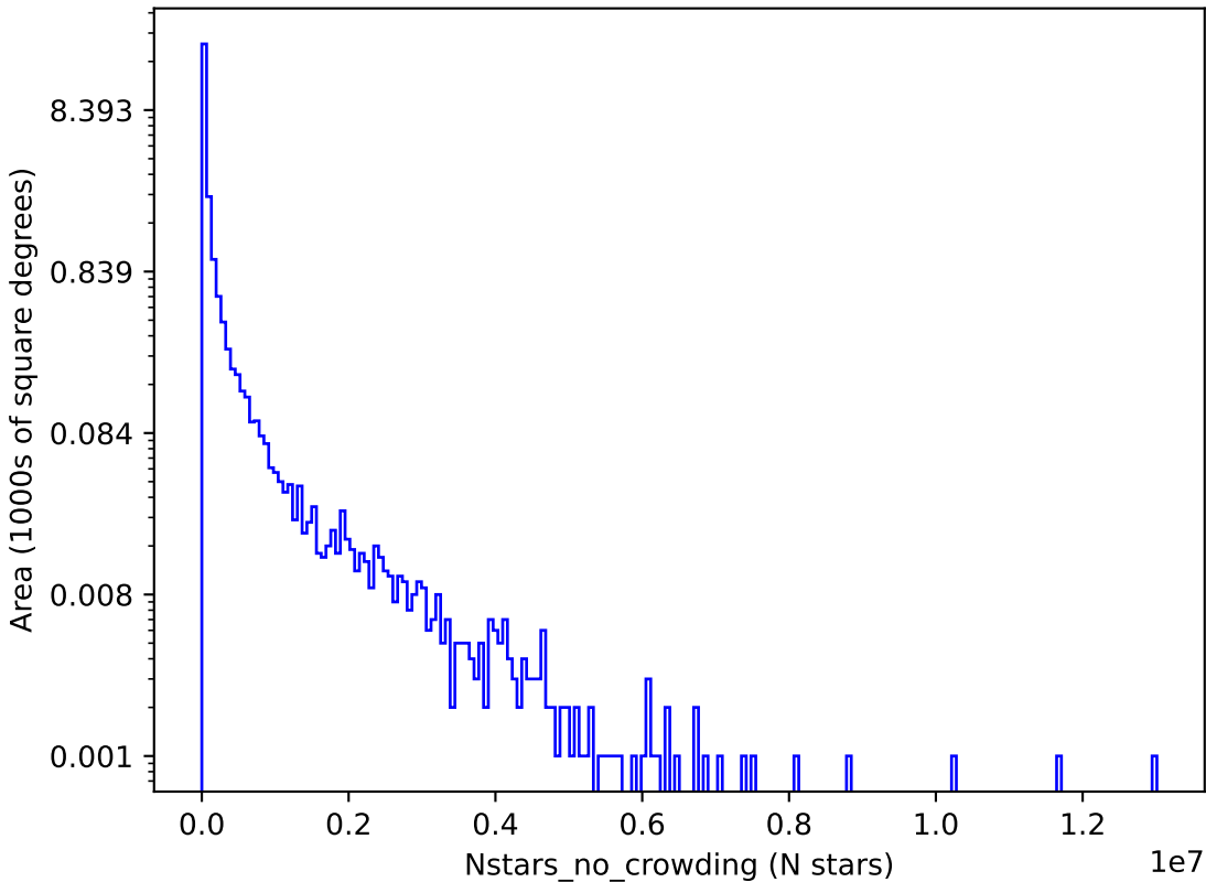
too_elab_r64_d3_gz_v3.4_10yrs g: Nstars_no_crowding
