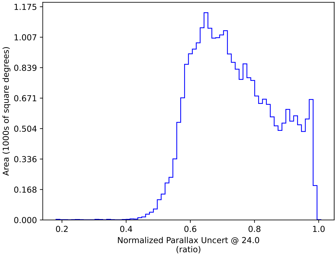
too_elab_r64_d3_gz_v3.4_10yrs : Normalized Parallax Uncert @ 24.0
