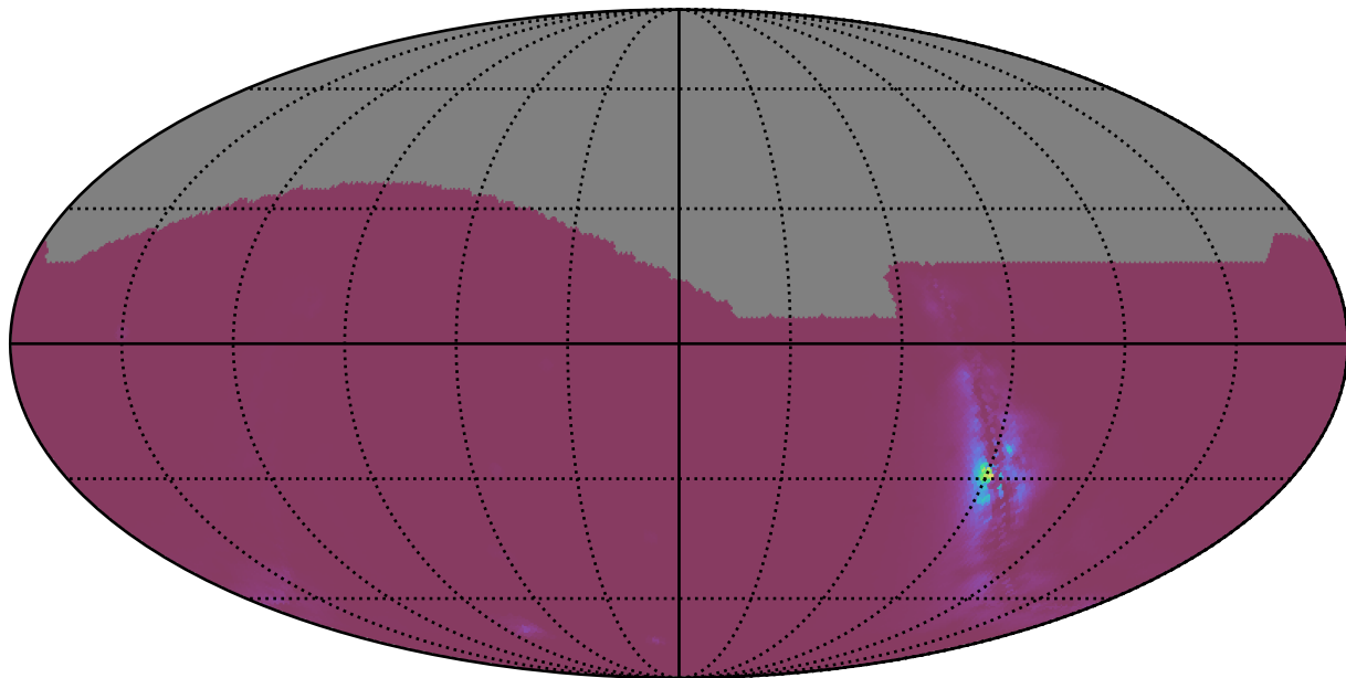
too_elab_r64_d3_gz_v3.4_10yrs : NlcPoints
