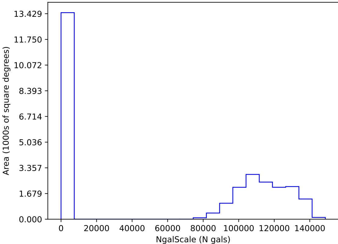
too_elab_r64_d3_gz_v3.4_10yrs i: NgalScale
