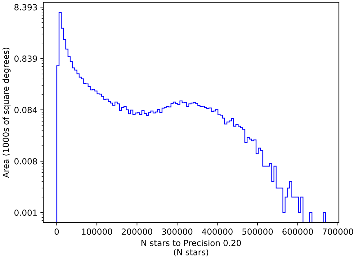
too_elab_r64_d3_gz_v3.4_10yrs y: N stars to Precision 0.20
