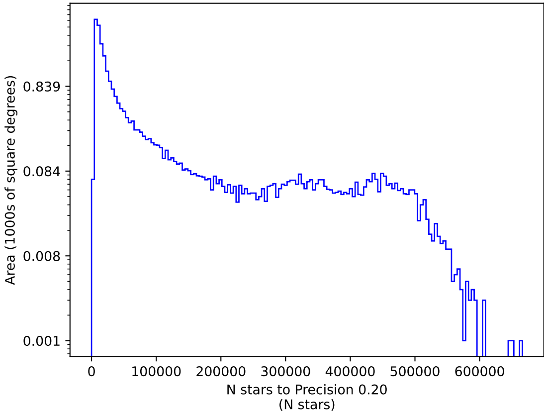
too_elab_r64_d3_gz_v3.4_10yrs r: N stars to Precision 0.20
