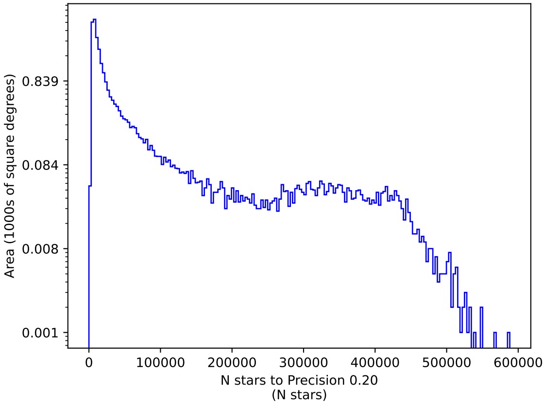
too_elab_r64_d3_gz_v3.4_10yrs g: N stars to Precision 0.20
