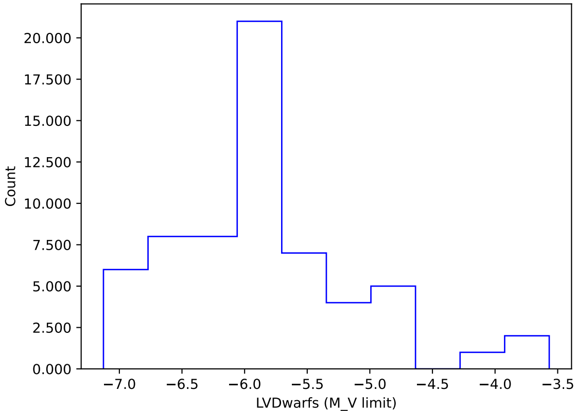
too_elab_r64_d3_gz_v3.4_10yrs gi: LVDwarfs
