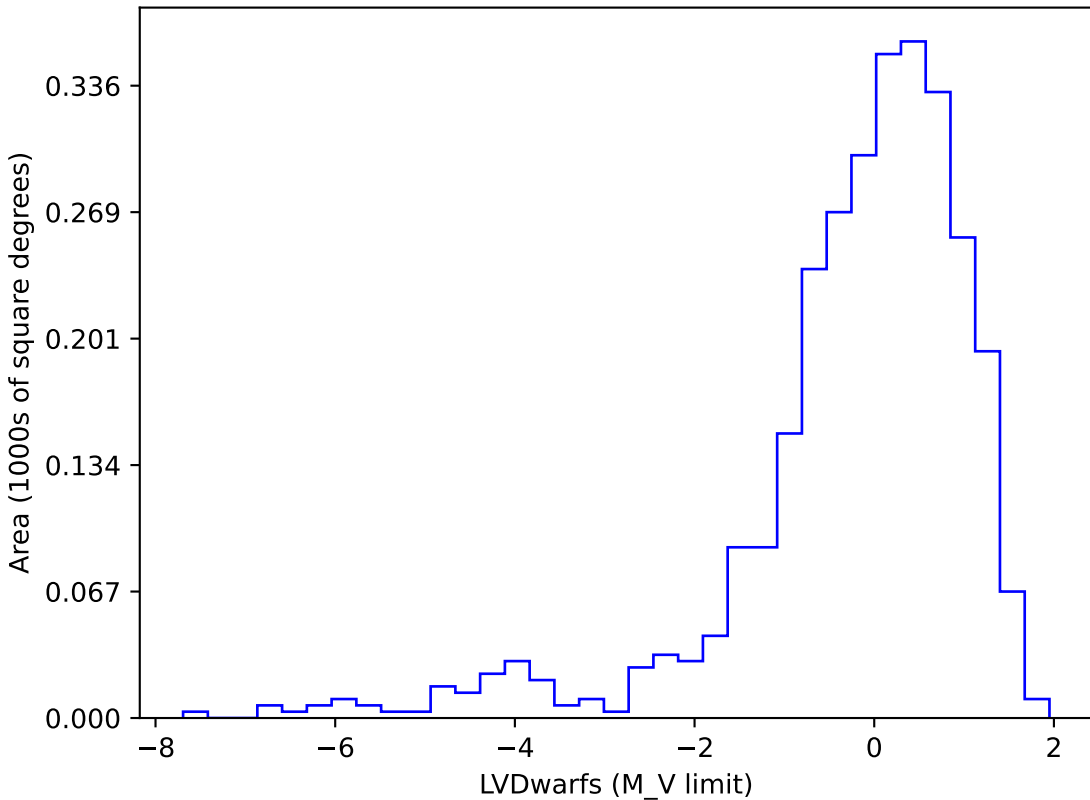
too_elab_r64_d3_gz_v3.4_10yrs gi SCP: LVDwarfs
