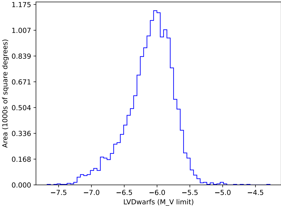
too_elab_r64_d3_gz_v3.4_10yrs gi: LVDwarfs
