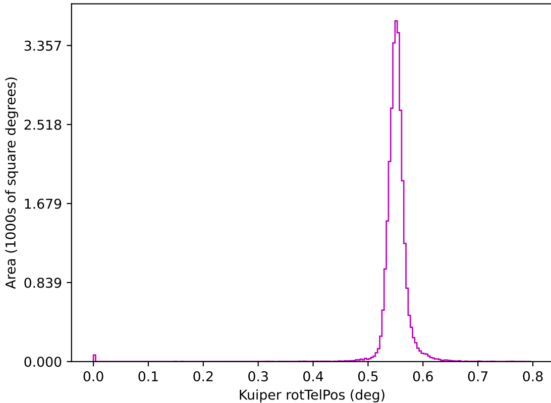
too_elab_r64_d3_gz_v3.4_10yrs z: Kuiper rotTelPos
