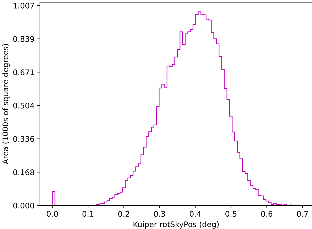
too_elab_r64_d3_gz_v3.4_10yrs z: Kuiper rotSkyPos
