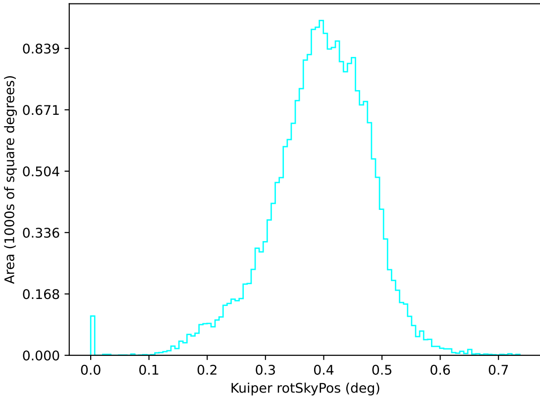
too_elab_r64_d3_gz_v3.4_10yrs u: Kuiper rotSkyPos
