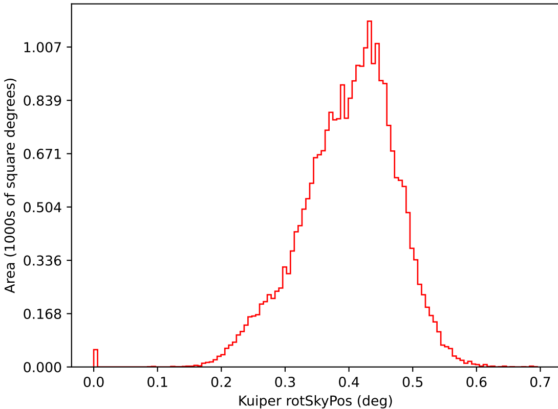
too_elab_r64_d3_gz_v3.4_10yrs i: Kuiper rotSkyPos
