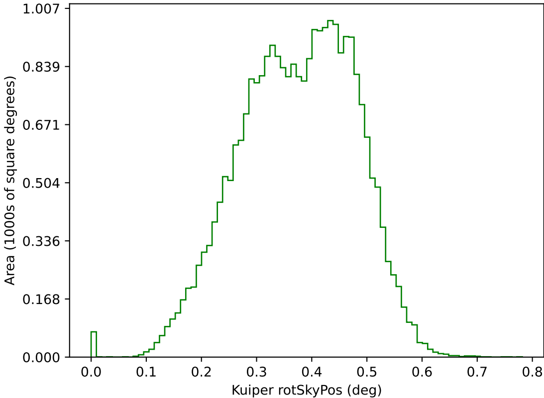
too_elab_r64_d3_gz_v3.4_10yrs g: Kuiper rotSkyPos
