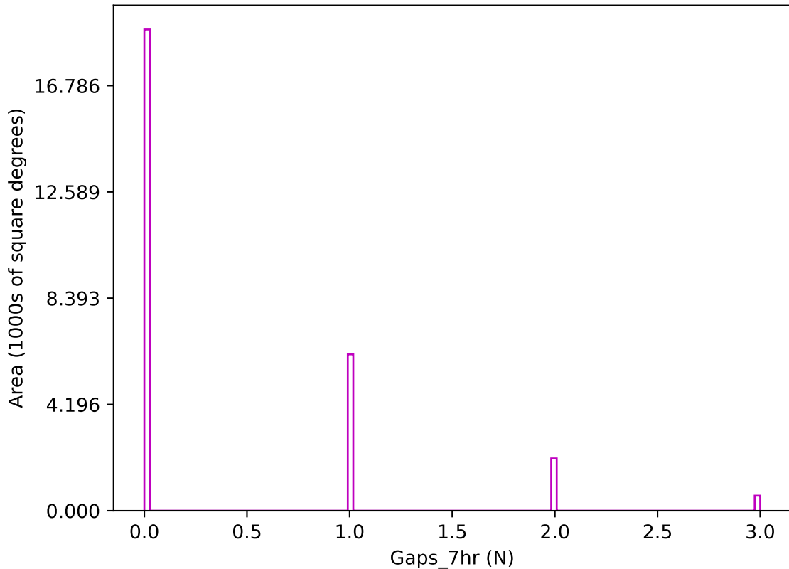
too_elab_r64_d3_gz_v3.4_10yrs z band: Gaps_7hr
