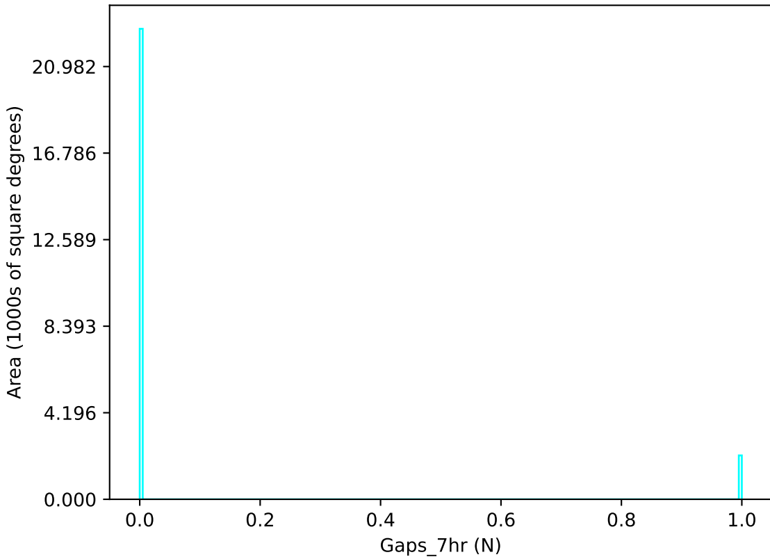
too_elab_r64_d3_gz_v3.4_10yrs u band: Gaps_7hr
