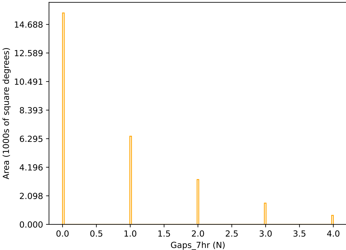
too_elab_r64_d3_gz_v3.4_10yrs r band: Gaps_7hr
