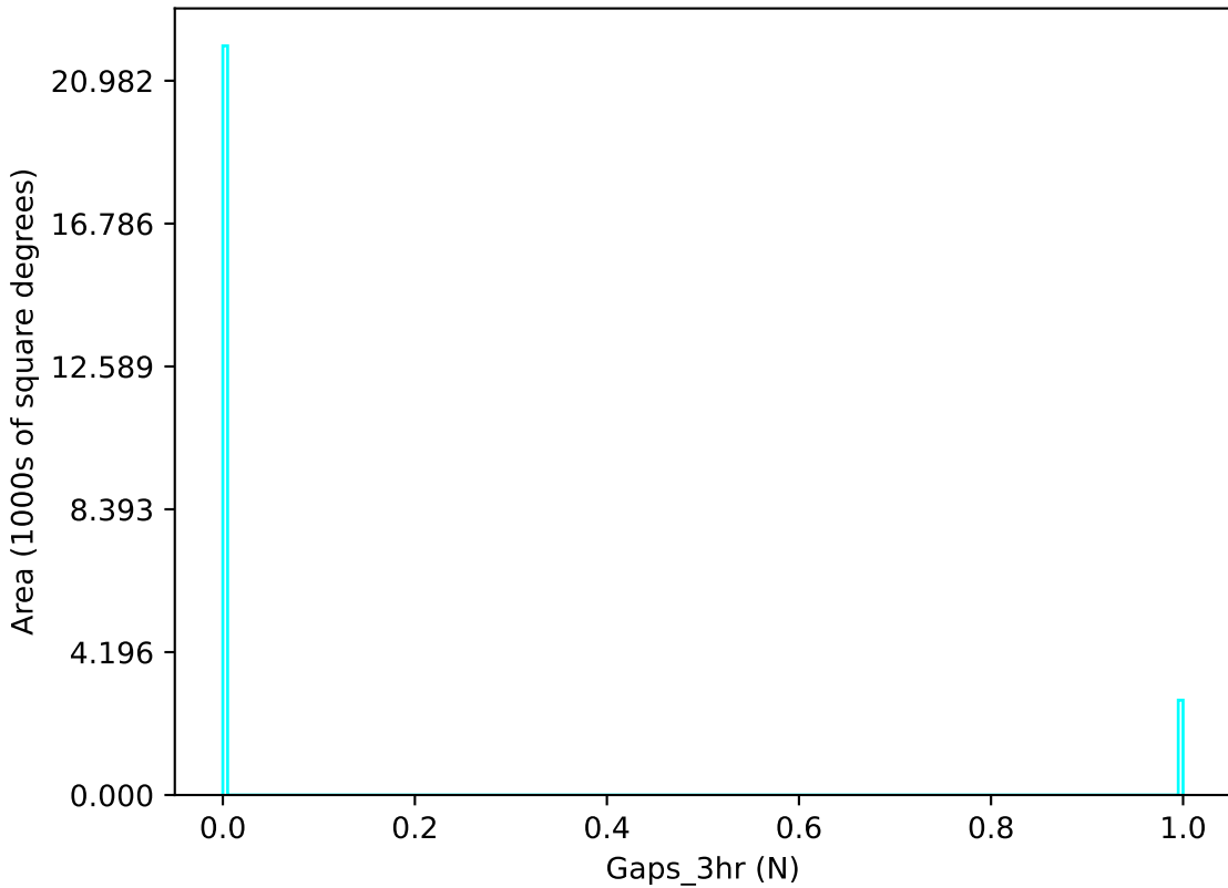
too_elab_r64_d3_gz_v3.4_10yrs u band: Gaps_3hr
