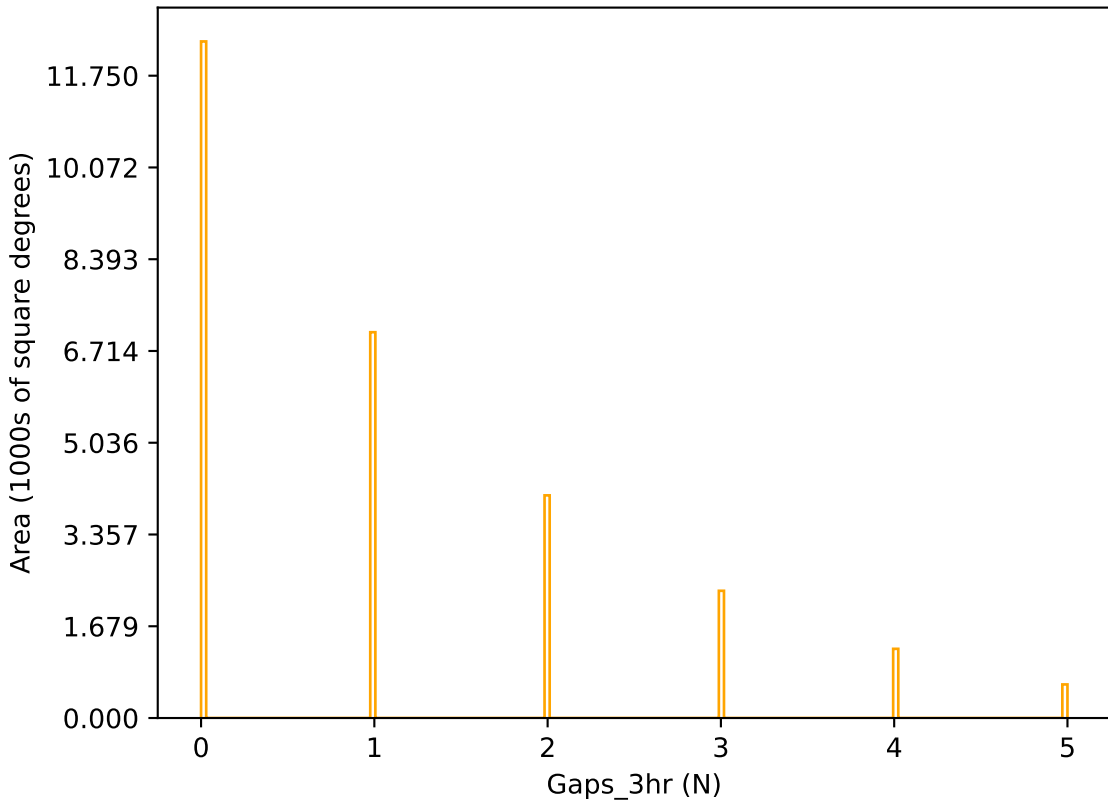
too_elab_r64_d3_gz_v3.4_10yrs r band: Gaps_3hr
