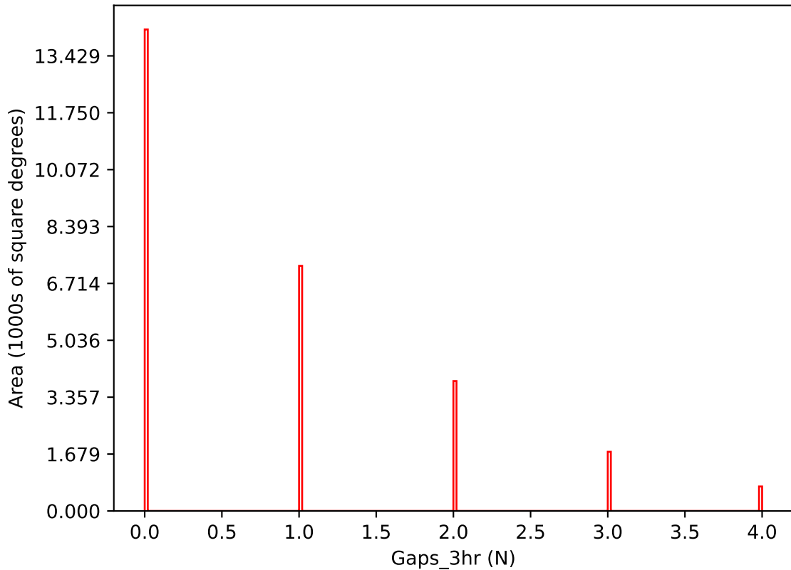
too_elab_r64_d3_gz_v3.4_10yrs i band: Gaps_3hr
