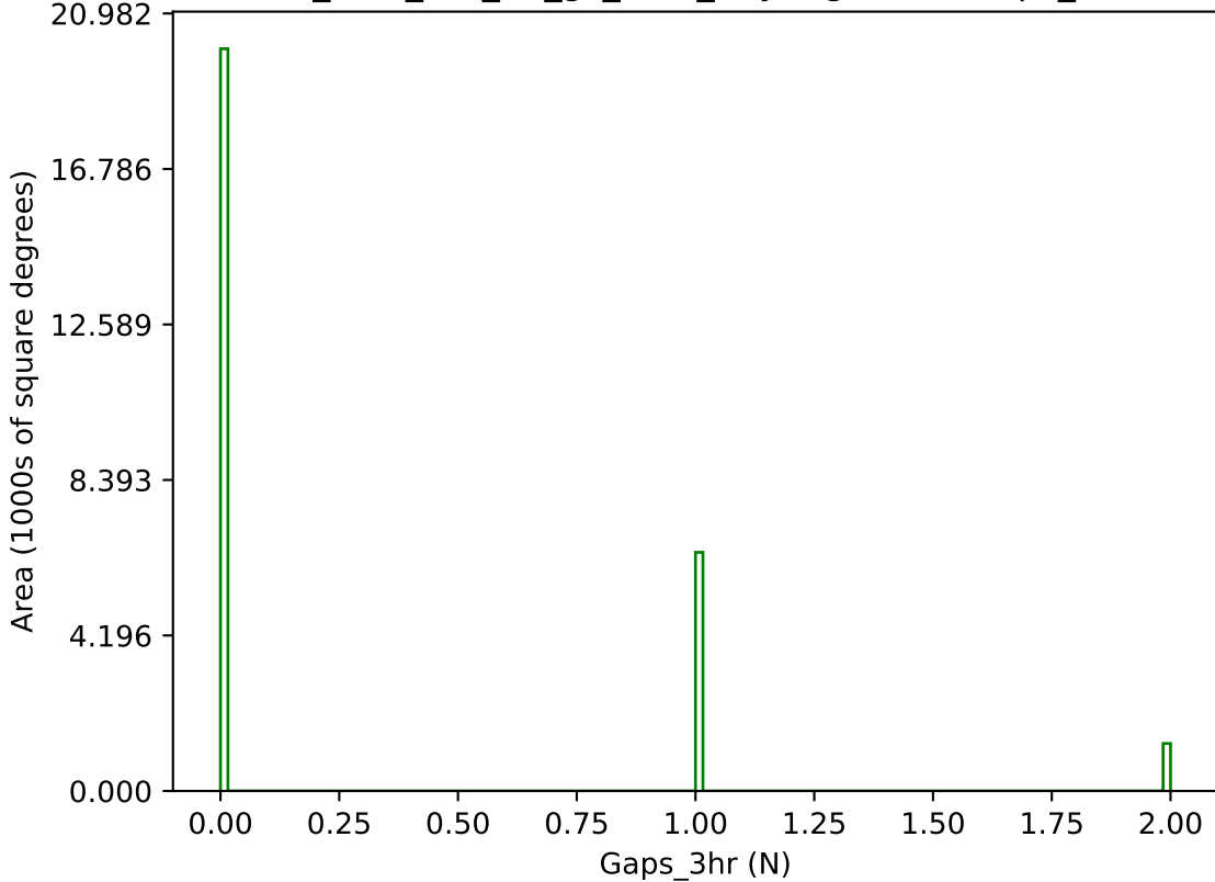
too_elab_r64_d3_gz_v3.4_10yrs g band: Gaps_3hr
