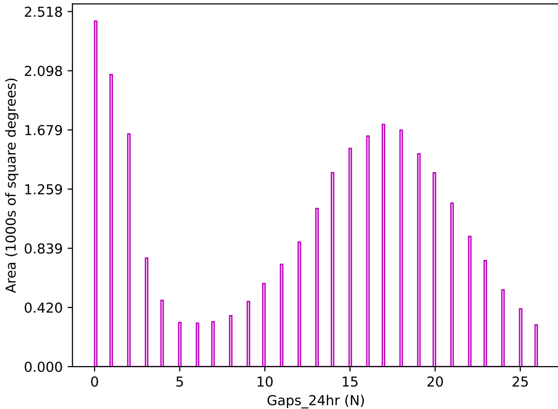
too_elab_r64_d3_gz_v3.4_10yrs z band: Gaps_24hr
