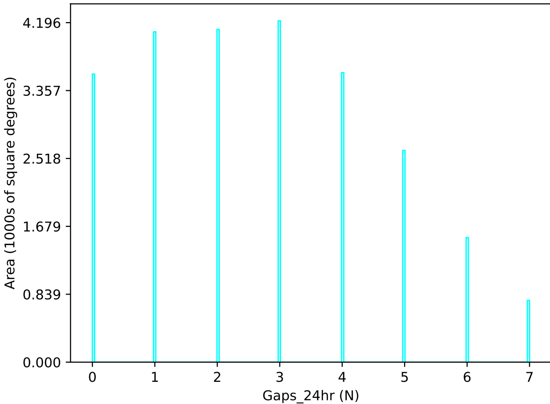
too_elab_r64_d3_gz_v3.4_10yrs u band: Gaps_24hr
