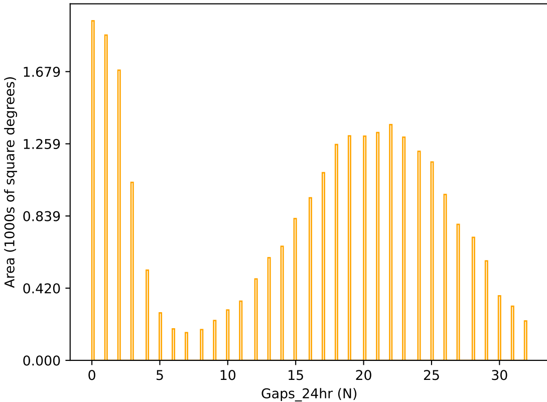
too_elab_r64_d3_gz_v3.4_10yrs r band: Gaps_24hr
