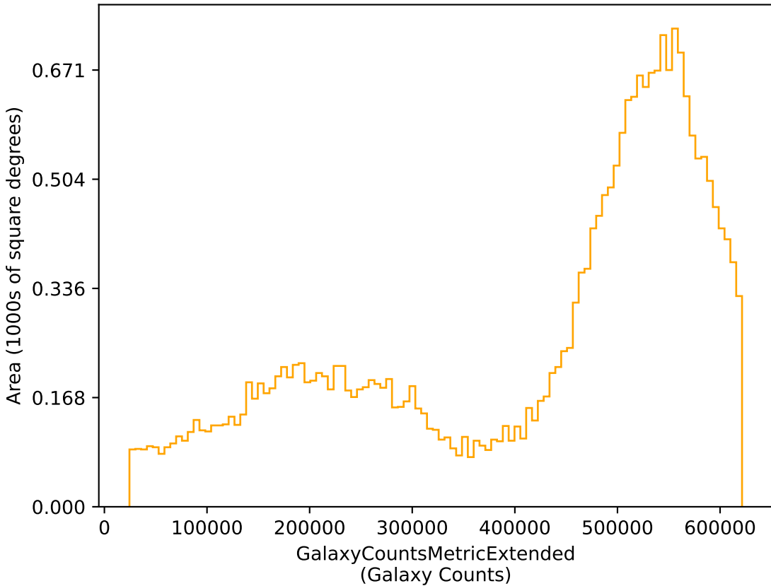
too_elab_r64_d3_gz_v3.4_10yrs r: GalaxyCountsMetricExtended
