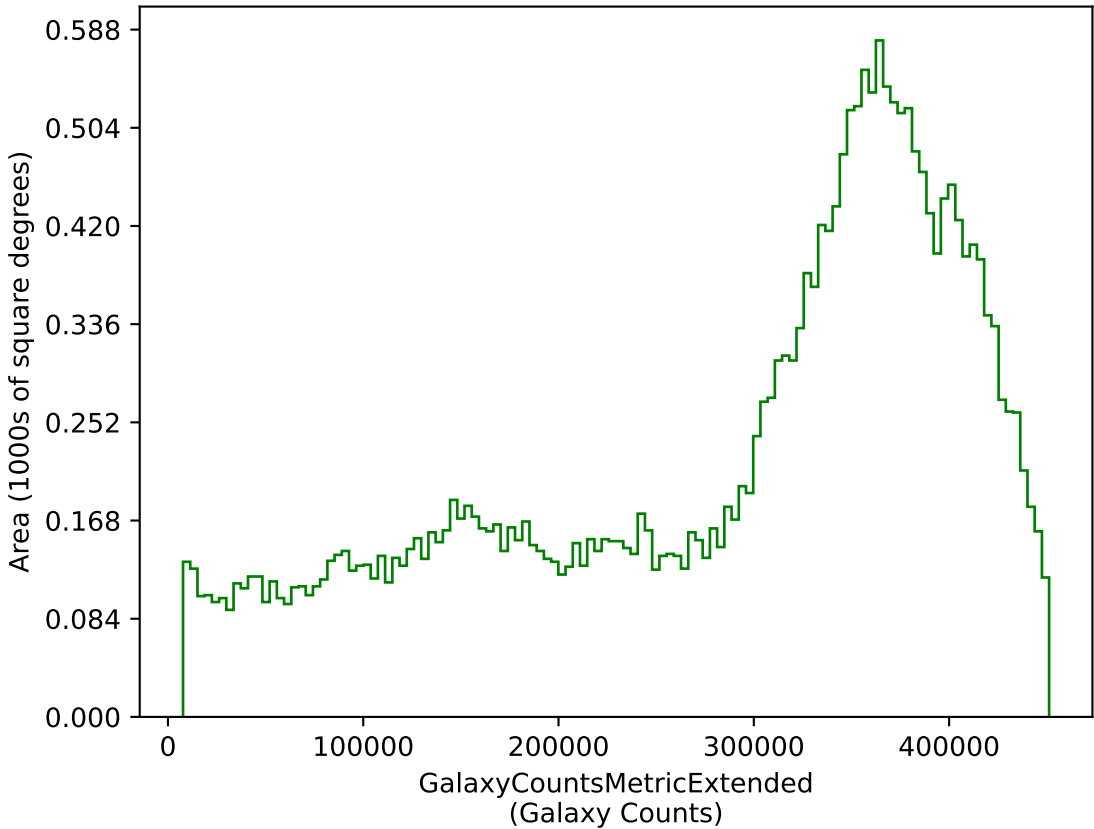
too_elab_r64_d3_gz_v3.4_10yrs g: GalaxyCountsMetricExtended
