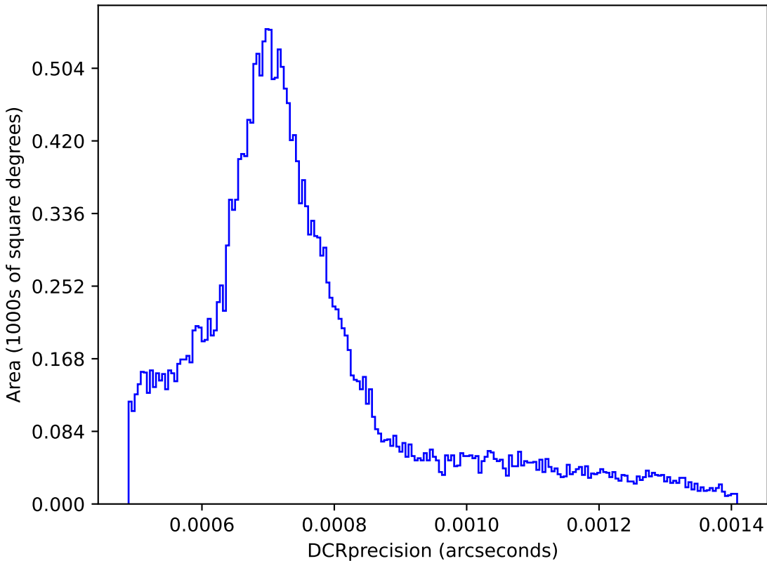
too_elab_r64_d3_gz_v3.4_10yrs : DCRprecision
