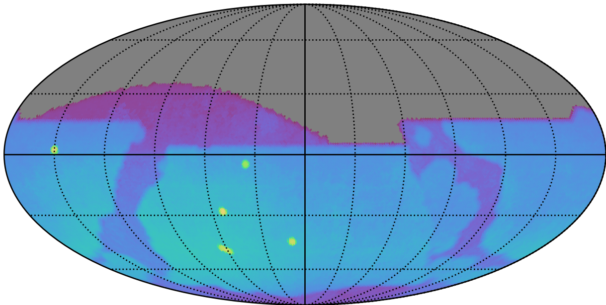
too_elab_r64_d3_gz_v3.4_10yrs : Brown Dwarf, L7
