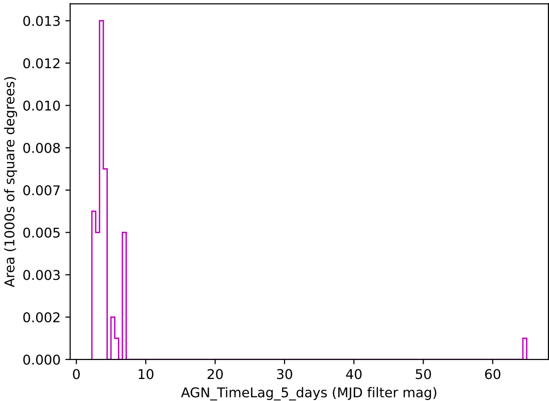
too_elab_r64_d3_gz_v3.4_10yrs z band: AGN_TimeLag_5_days
