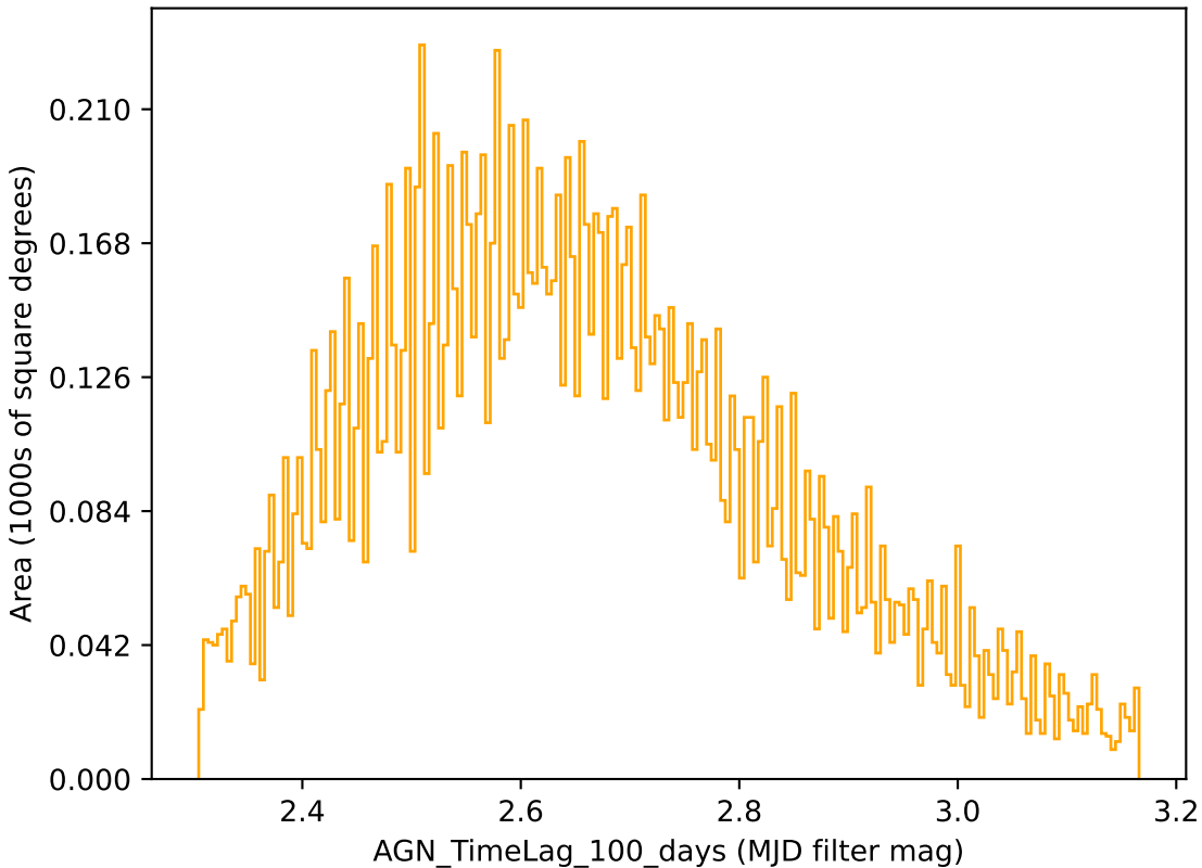
too_elab_r64_d3_gz_v3.4_10yrs r band: AGN_TimeLag_100_days
