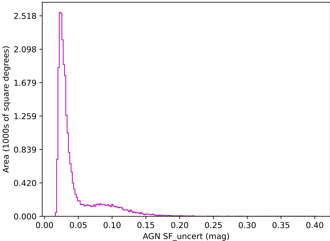
too_elab_r64_d3_gz_v3.4_10yrs z band: AGN SF_uncert
