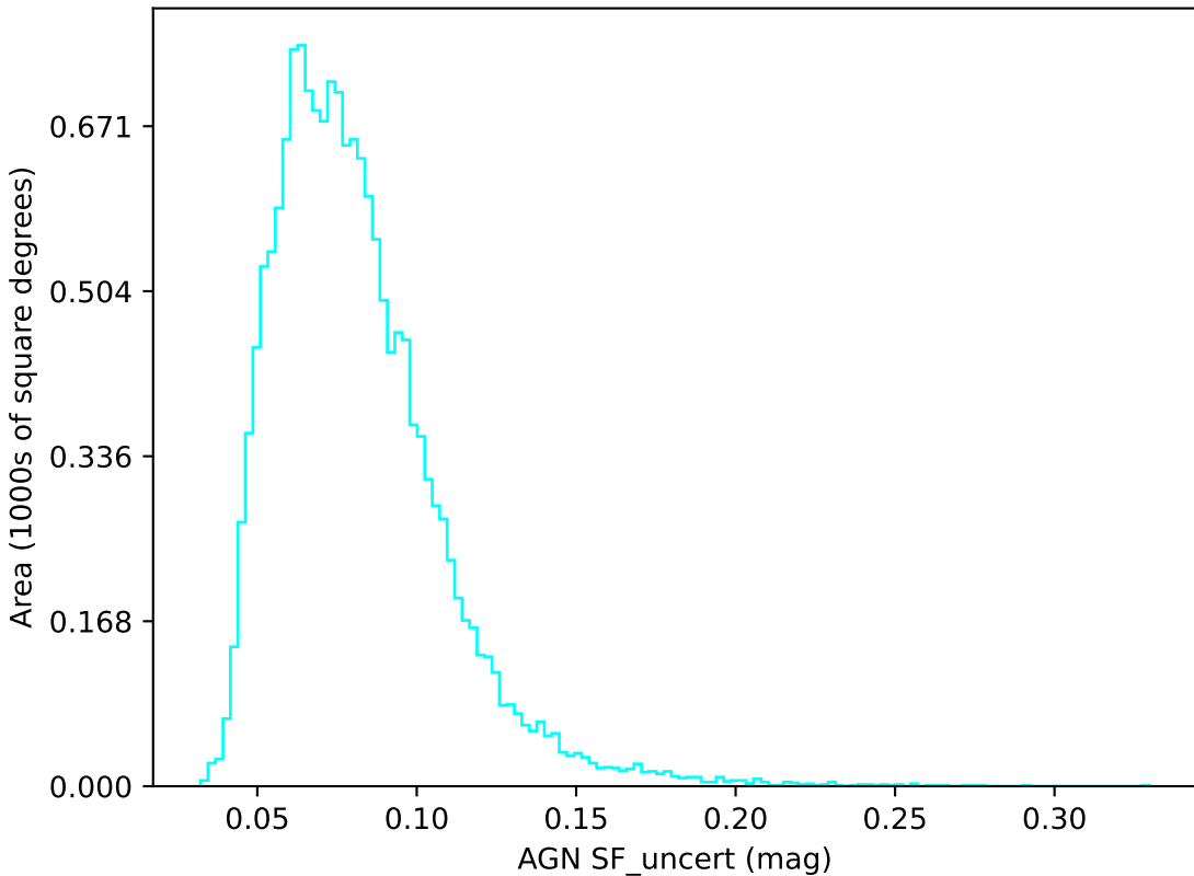
too_elab_r64_d3_gz_v3.4_10yrs u band: AGN SF_uncert
