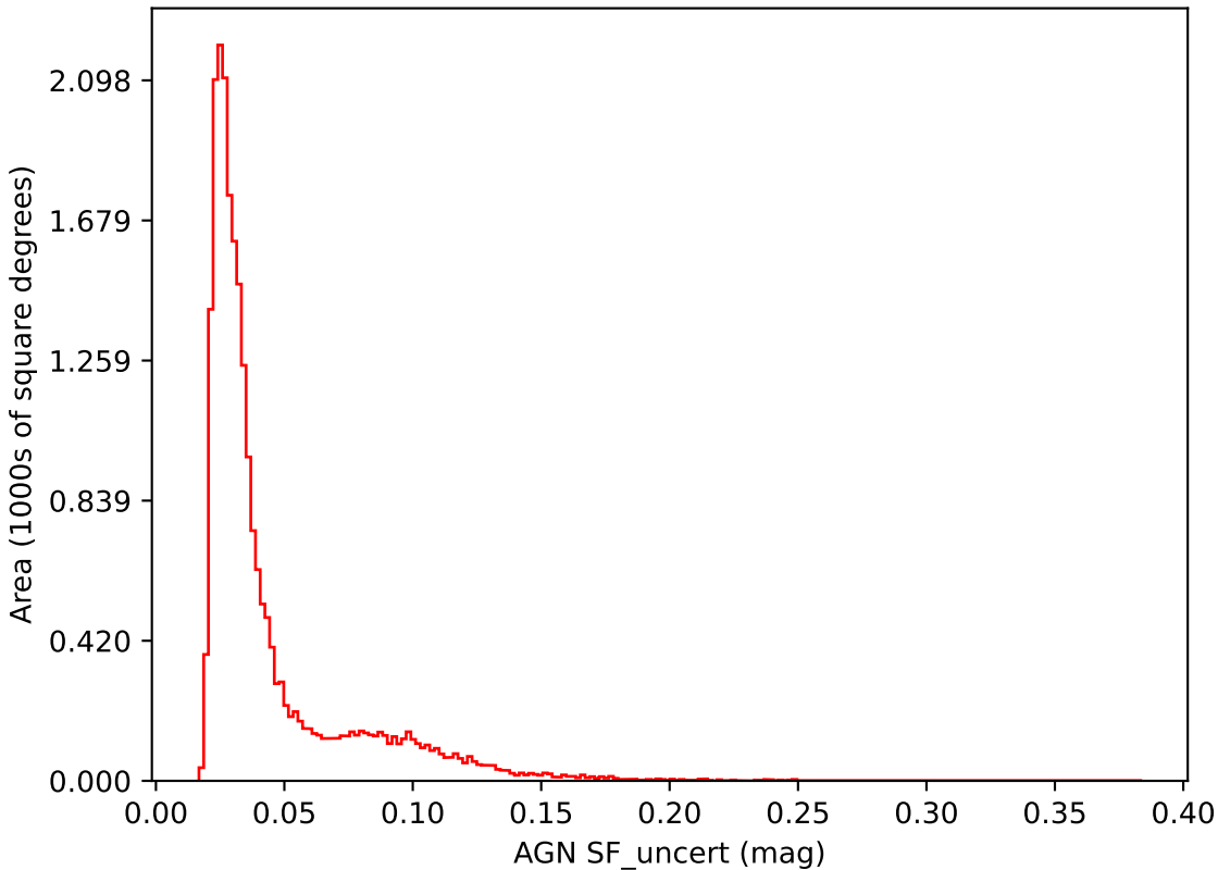
too_elab_r64_d3_gz_v3.4_10yrs i band: AGN SF_uncert
