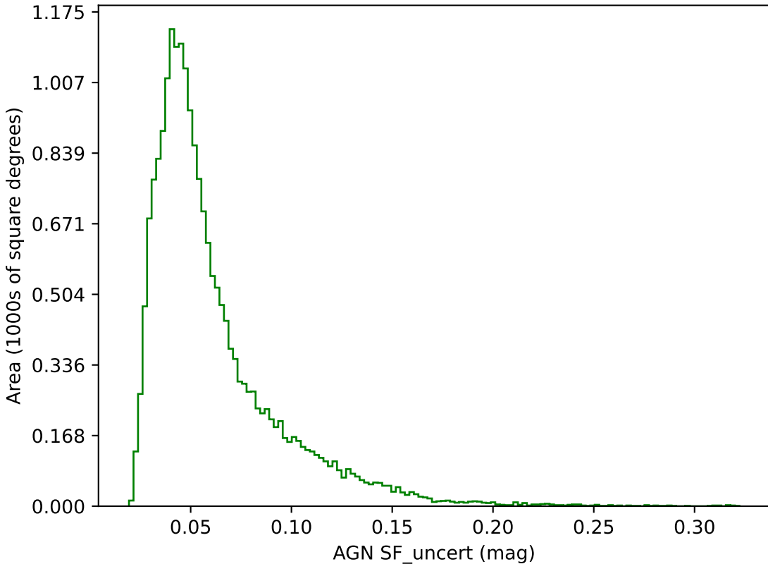
too_elab_r64_d3_gz_v3.4_10yrs g band: AGN SF_uncert
