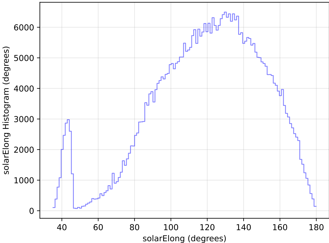
too_elab_r64_d3_gz_v3.4_10yrs WFD z band: solarElong Histogram
