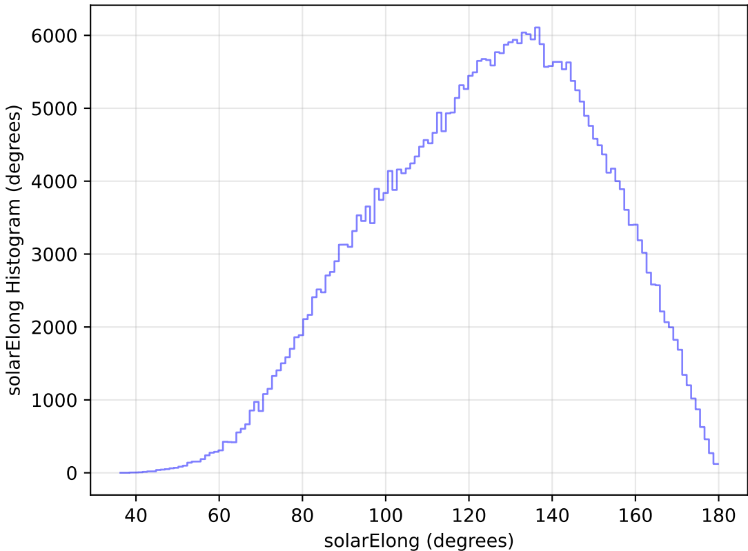
too_elab_r64_d3_gz_v3.4_10yrs WFD y band: solarElong Histogram
