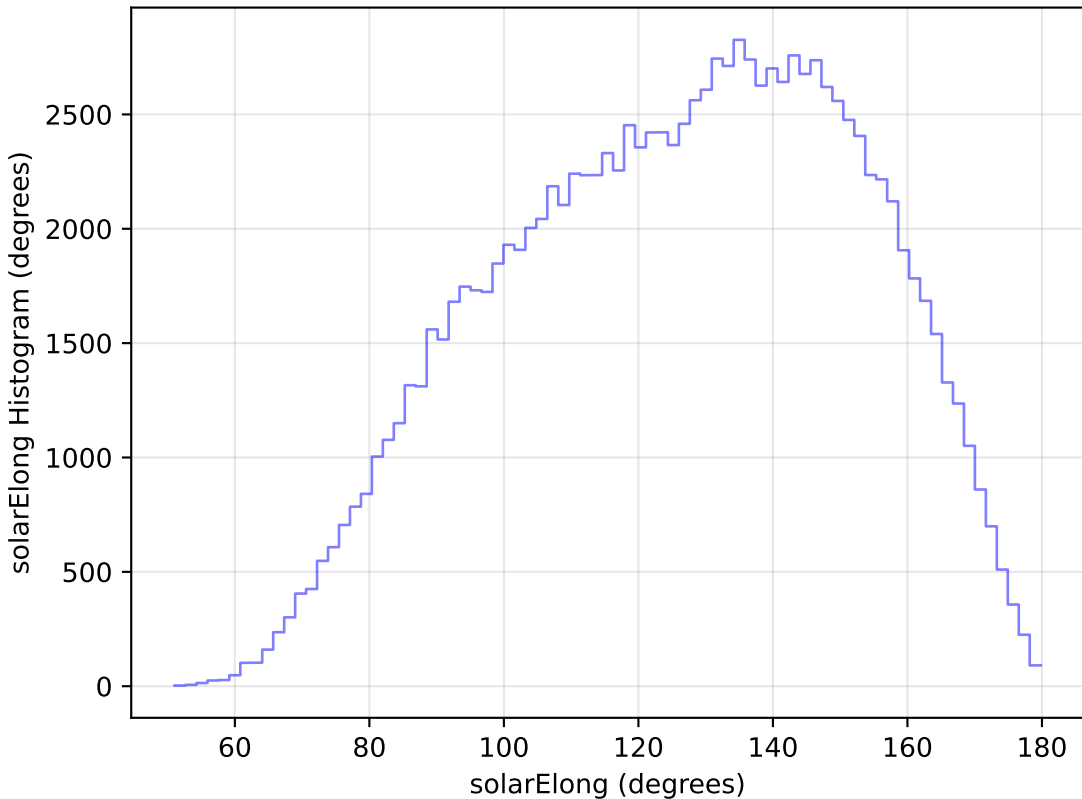
too_elab_r64_d3_gz_v3.4_10yrs WFD u band: solarElong Histogram
