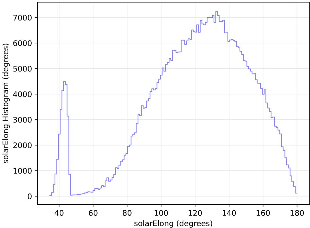
too_elab_r64_d3_gz_v3.4_10yrs WFD i band: solarElong Histogram
