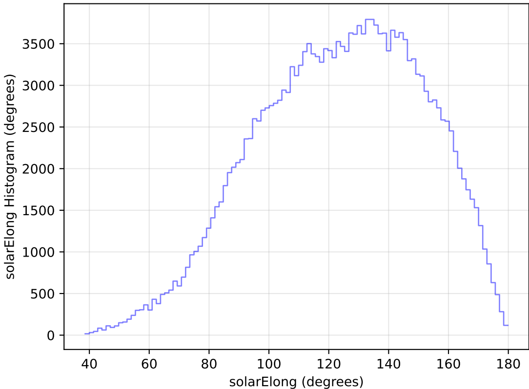
too_elab_r64_d3_gz_v3.4_10yrs WFD g band: solarElong Histogram
