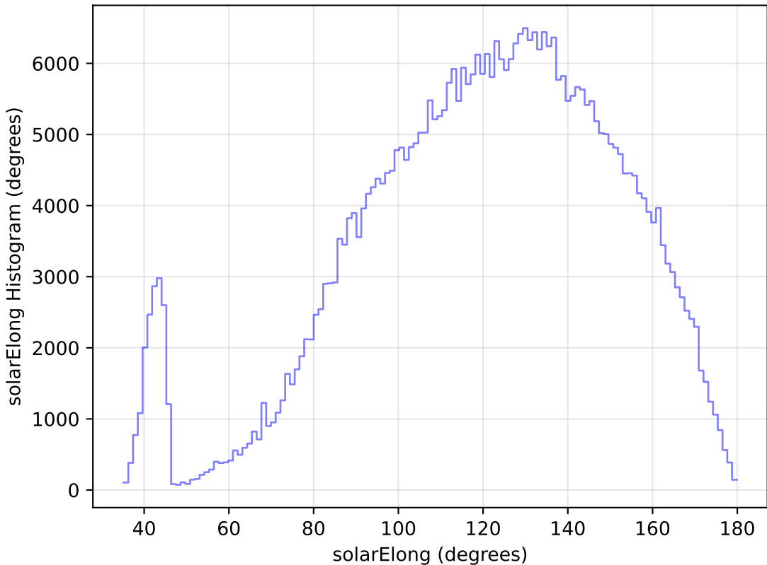
too_elab_r64_d3_gz_v3.4_10yrs All sky z band: solarElong Histogram
