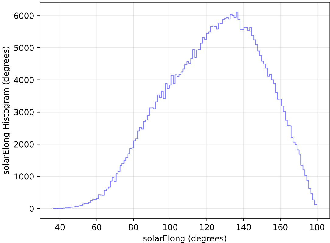
too_elab_r64_d3_gz_v3.4_10yrs All sky y band: solarElong Histogram
