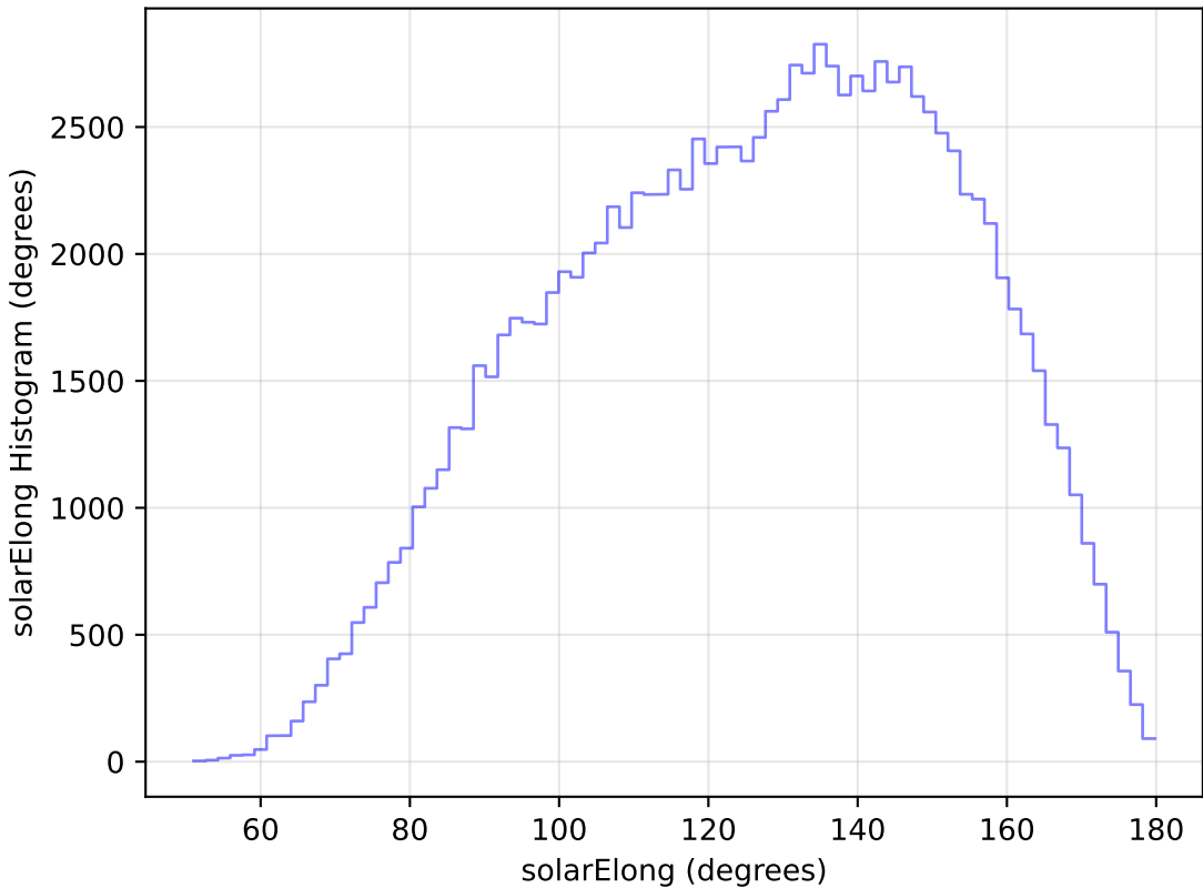
too_elab_r64_d3_gz_v3.4_10yrs All sky u band: solarElong Histogram
