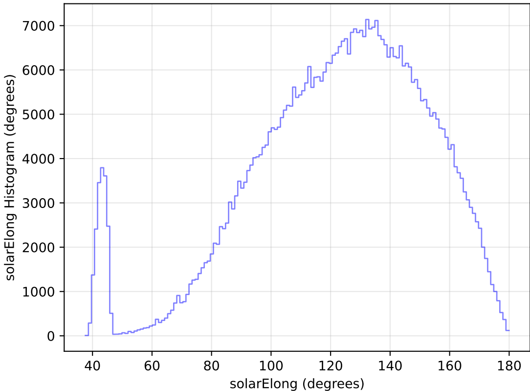
too_elab_r64_d3_gz_v3.4_10yrs All sky r band: solarElong Histogram
