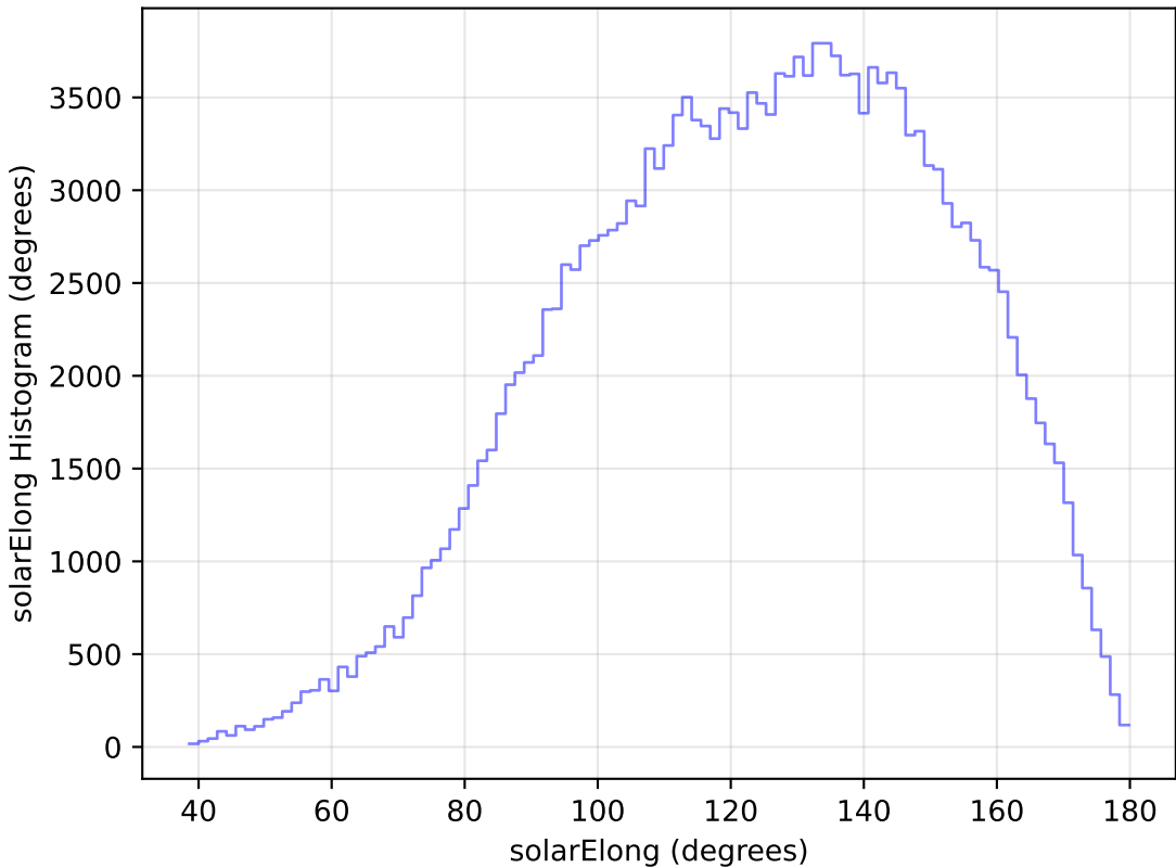
too_elab_r64_d3_gz_v3.4_10yrs All sky g band: solarElong Histogram
