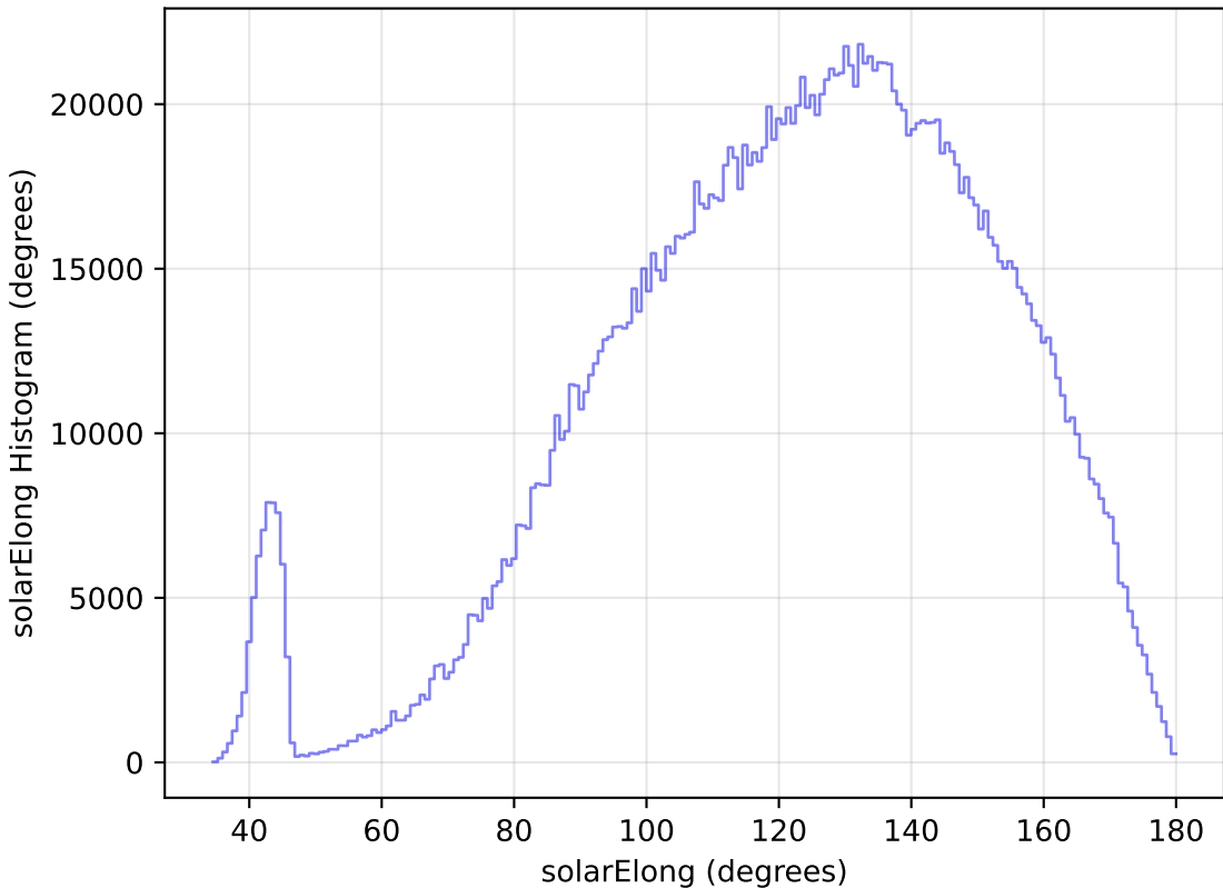
too_elab_r64_d3_gz_v3.4_10yrs All sky all bands: solarElong Histogram
