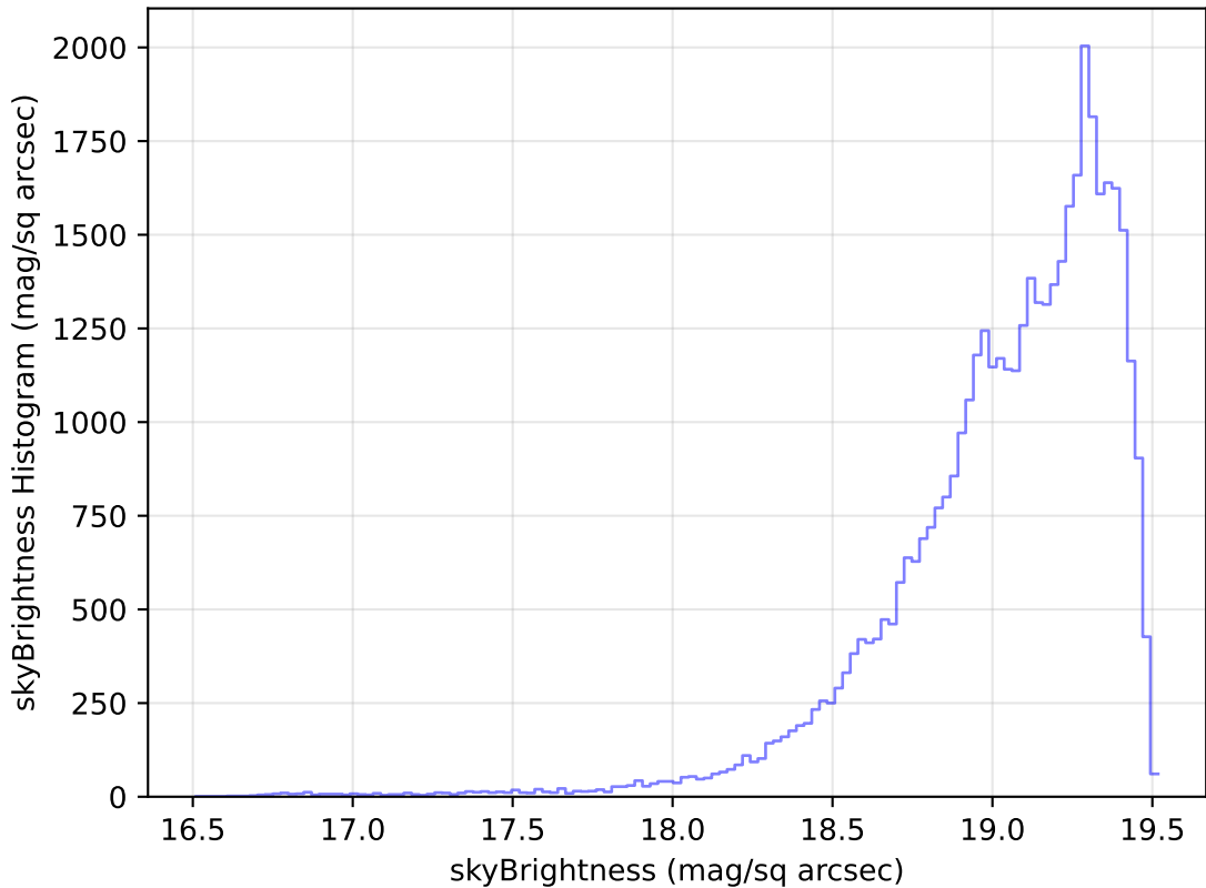
too_elab_r64_d3_gz_v3.4_10yrs Yr 1 z band: skyBrightness Histogram
